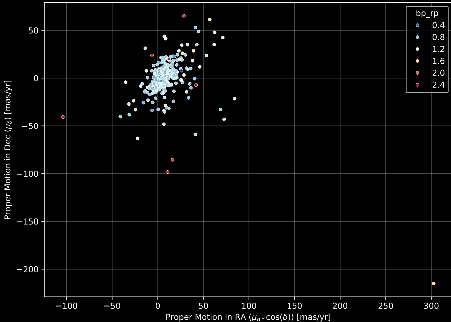
GALAH DR4 Field: [6883] Proper Motion Diagram (n= 294)
