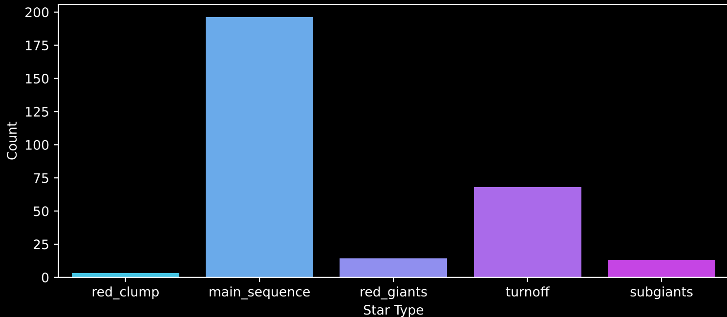
GALAH DR4 Field: [6883] Count plot of Star Type
