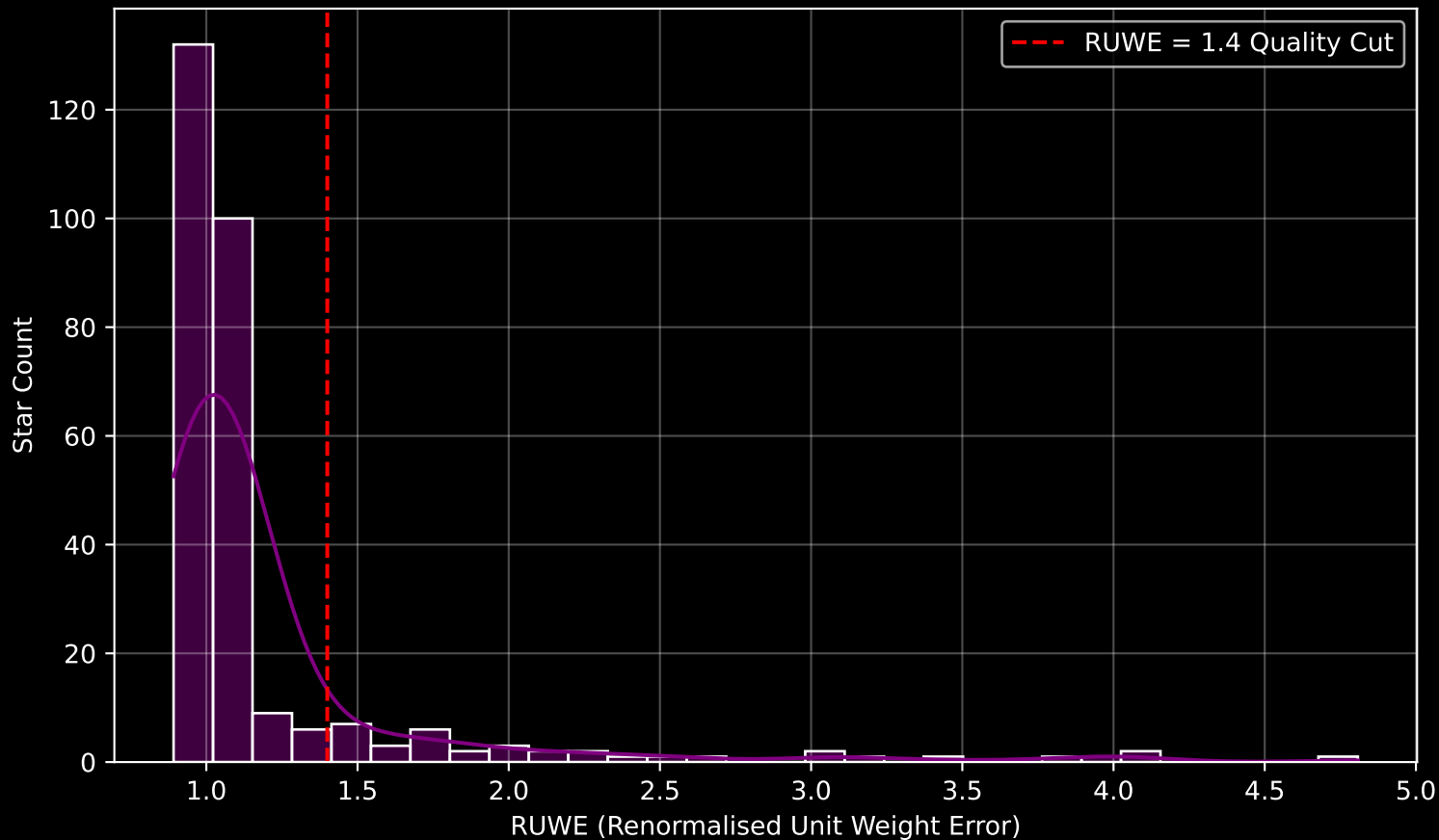
GALAH DR4 Field [6883] RUWE Distribution (n= 284)
